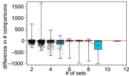
Fig. 9. Extrapolate Ahead ( l = \sqrt{n_i} ) (low wins) vs. Interpolation Small Adaptive (high wins). Deterioration of performance for a polynomial look-ahead range.
