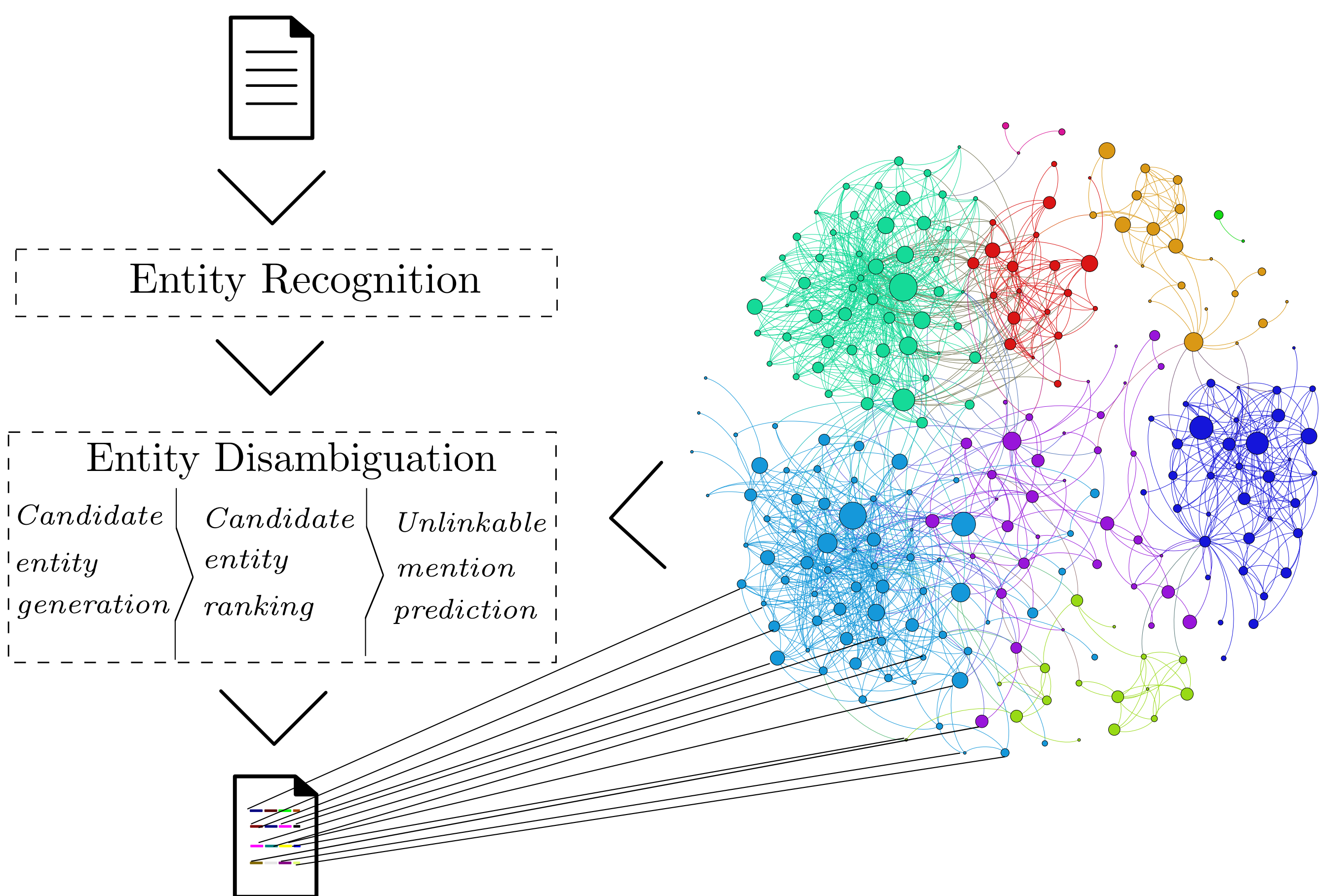
Fig 2. Entity Linking Flow
