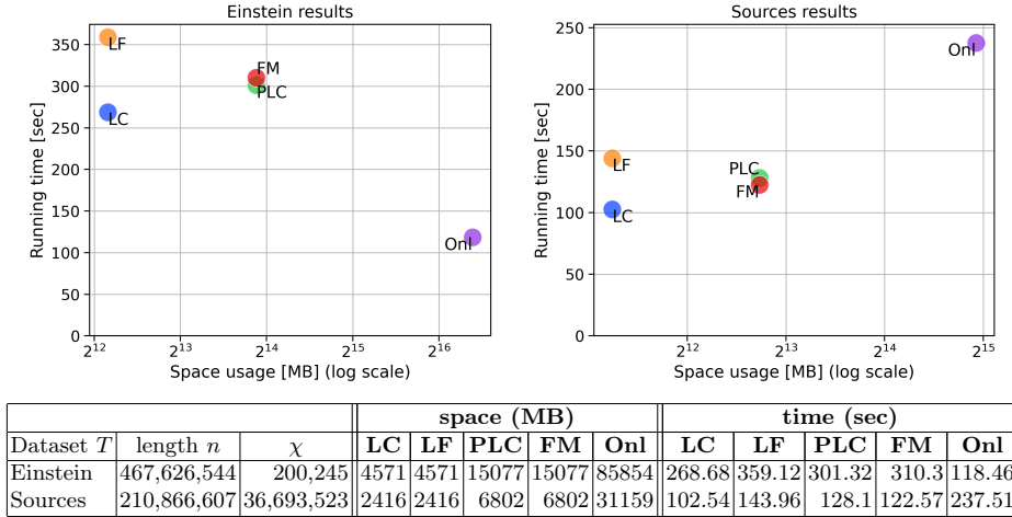
Fig. 2. Space usage and running time comparison between all construction algorithms on einstein.en.txt and sources sequences from Pizza&Chili collection. Logscale in the space coordinate.
