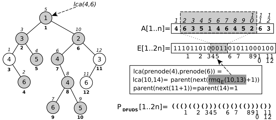
Figure 2: The same arrangement of Figure 1, now on the DFUDS representation of the Cartesian tree. The query \text{rmq}_A(2, 10) becomes \text{lca}(4, 6) , which we translate into \text{lca}(10, 14) when the node identifiers become positions in DFUDS instead of preorders (the translation is shown on the bottom of the sequence P_{\text{DFUDS}} ).
