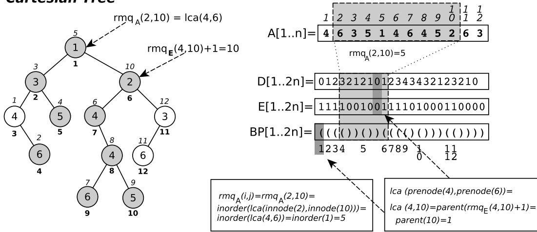
Figure 1: An example array A[1, 12] (top right) and its Cartesian tree (left). We choose preorder numbers as node identifiers (in bold under the nodes), and also write inorder values on top of the nodes, in slanted font. The left rectangle on the bottom shows how query \text{rmq}_A(2, 10) translates into query \text{lca}(4, 6) on the Cartesian tree. We also show how this query, in turn, maps into \text{rmq}_D(4, 10) , on the array D of depths of the tree. Array E tells if consecutive entries of D increase or decrease, and is the same as a BP representation of the tree. The right rectangle on the bottom shows how query \text{lca}(4, 10) is solved using \text{rmq}_E(4, 10) and \text{parent} on the parentheses. This \text{rmq}_E query is a simpler \pm 1 -RMQ problem. Now the nodes 4, 10, and 1 do not refer to preorders but to positions in BP, obtained from preorders with \text{prenode} . The corresponding preorder values are written below the BP array.
