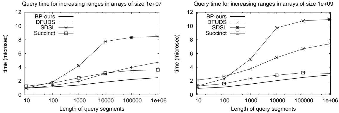
Figure 5: Query time on random arrays, for ranges of increasing size and two values of n .
