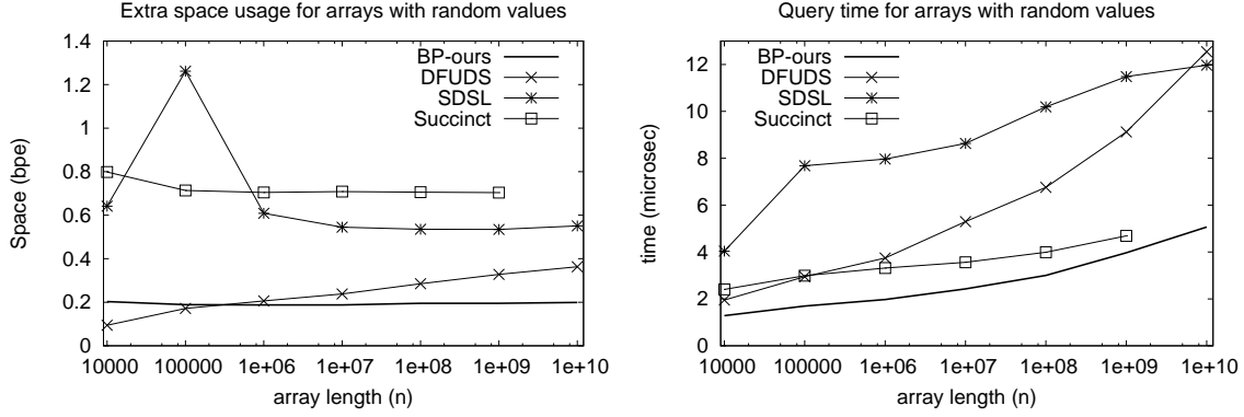
Figure 4: Query space and time on random arrays, for ranges of size 10,000.
