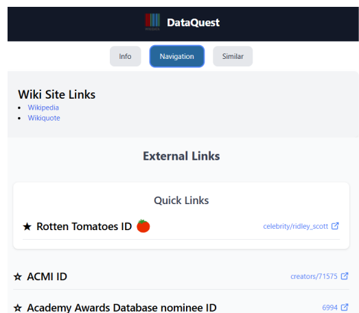
Figure 2: Navigation tab of DATAQUEST
