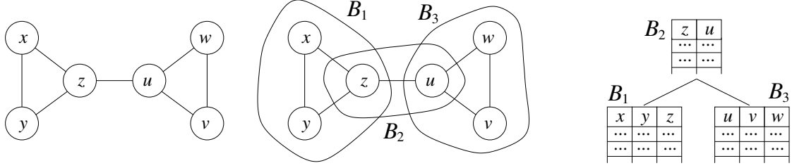
Figure 1: On the left, a barbell BGP with 6 variables. In the middle, a GHD decomposition into 3 bags. On the right, a join tree on the resulting tables, to apply Yannakakis’ algorithm.
