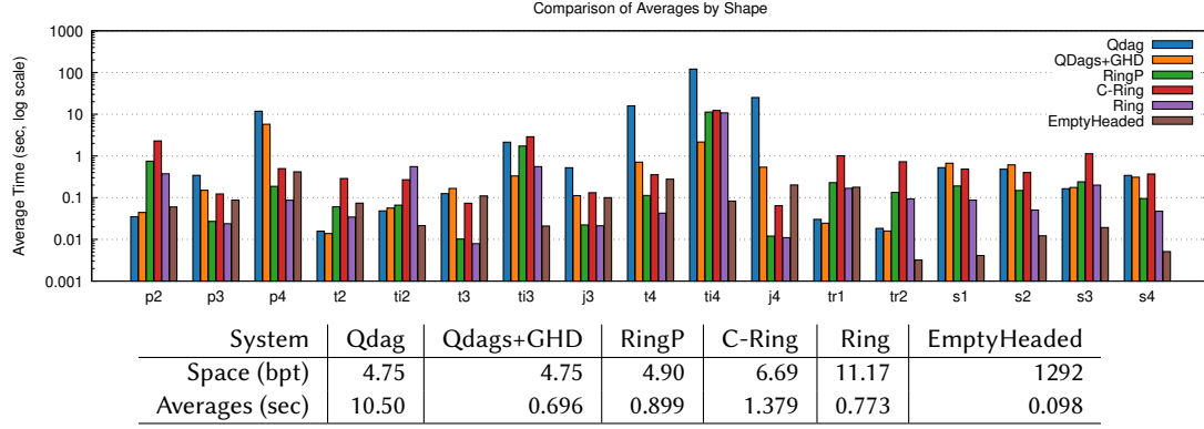
Figure 8: Average times for various systems, for the different shapes. Below, space (in bytes per triple) and global averages over all shapes.
