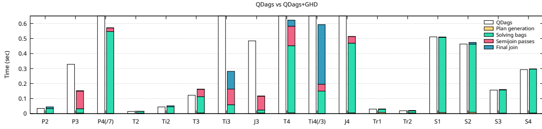
Figure 7: Average times breakdown, in seconds, of original (white) versus our improved Qdags. For legibility, P4 times are divided by 7 (QDags time is 10.6) and Ti4 times are divided by 3.
