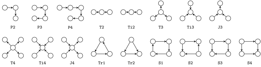
Figure 4: The 17 query shapes tested on the Wikidata graph.
