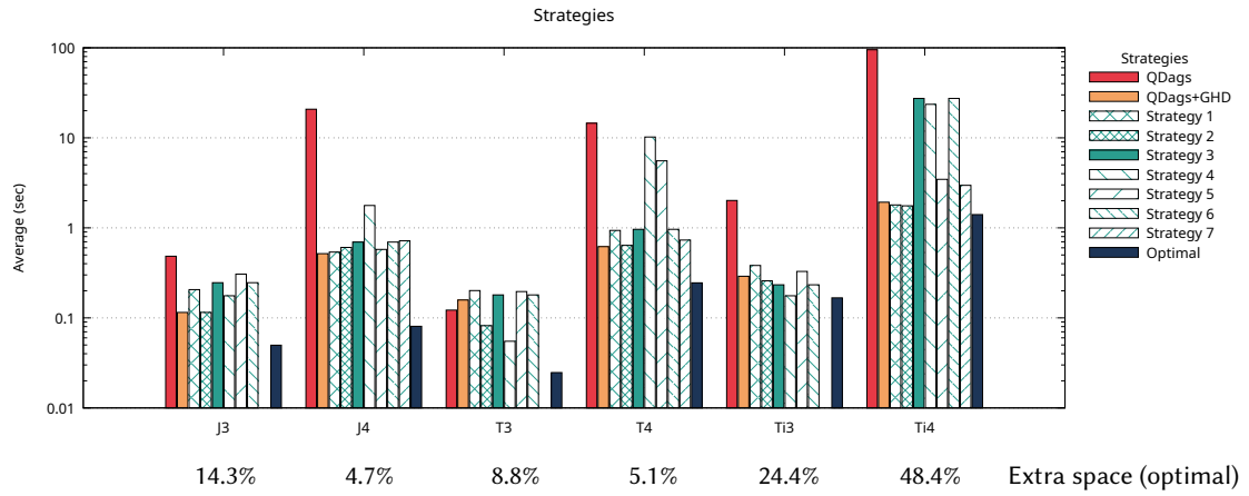
Figure 5: Average times, in seconds, of original versus our improved QDags. Logscale.
